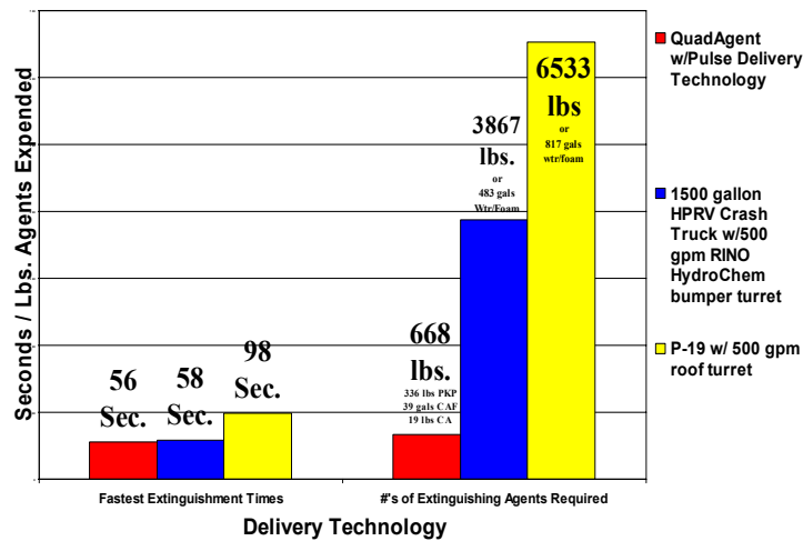
Delivery Technology Comparison Chart 100' Diameter Pit with Aircraft Simulator w/1000 gals JP fuel
